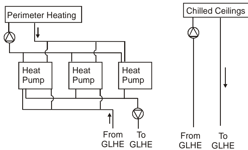
Figure 2: Direct Cooling GSHP System
