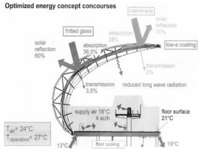
Figure 8 Optimized energy concept concourses for SBIA.
