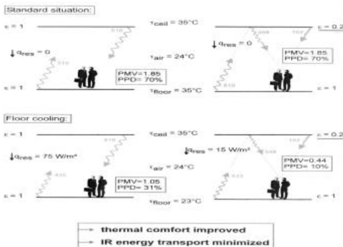
Figure 1 The effect of low emission IR coating.
