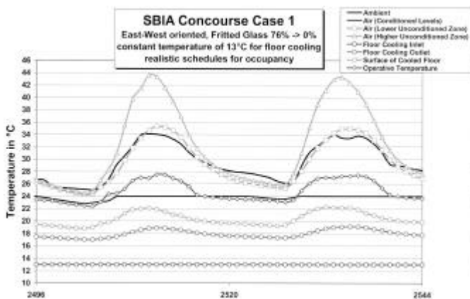
Figure 3 SBIA concourse, case 1.
