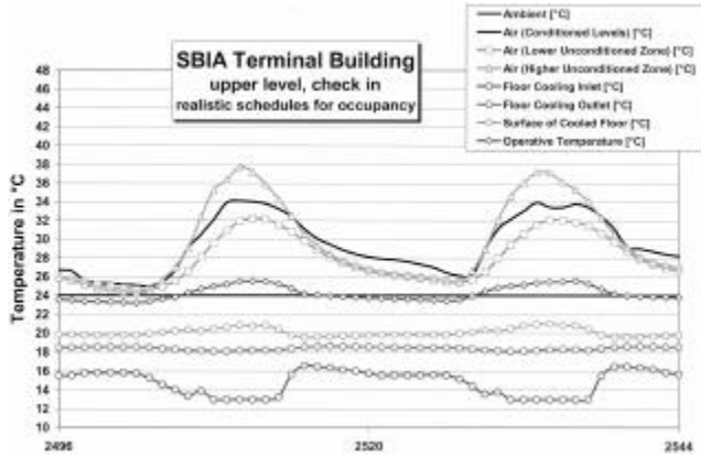
Figure 6 SBIA terminal building upper level.
