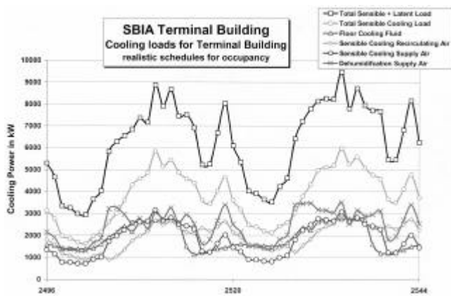
Figure 5 SBIA terminal building cooling loads.
