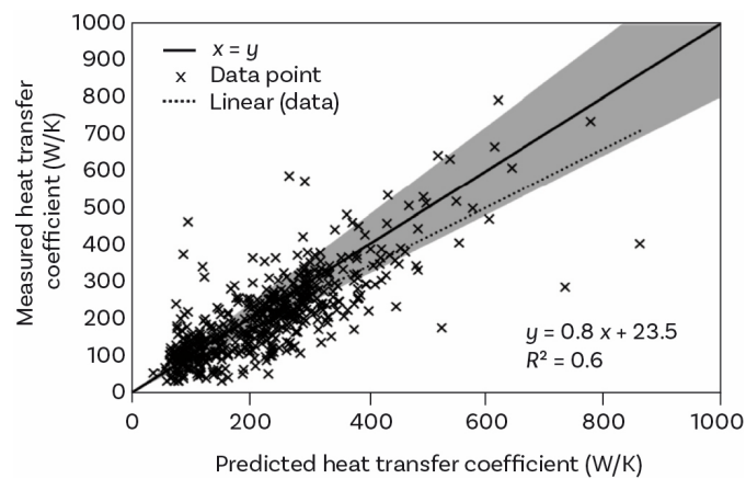
Figure 3 Comparison between calculated and measured HTC's (BTS, online a). Points within the shaded area have calculated performance within the confidence interval of the measurement, those above the solid x = y line have worse measured performance than calculated.
